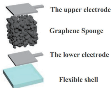
Fig. 1. The schematic diagram of structure of the flexible sensor.
